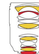
Optical Construction : 14 elements in 10 groups Filter Size : ø72mm Length : 102.3mm (4in) Weight : 805g (28.4oz) Minimum Object Distance : 0.3m (11.8in)
