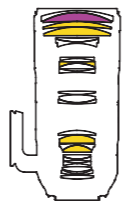
Optical Construction : 23 elements in 17 groups Filter Size : ø77mm Length : 191.3mm (7.5in) Weight : 1,385g (48.9oz) (without tripod mount) / tripod mount 100g (3.5oz) Minimum Object Distance : 0.95m (37.4in)
